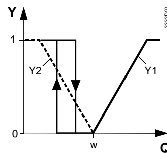
1-stage cooling
